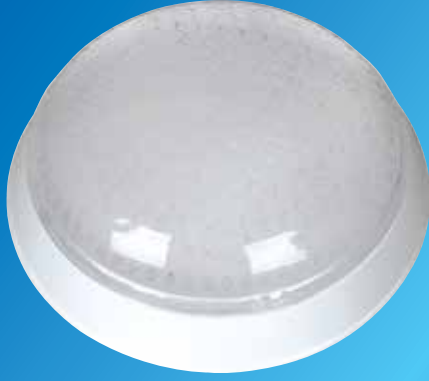
Luna 5
